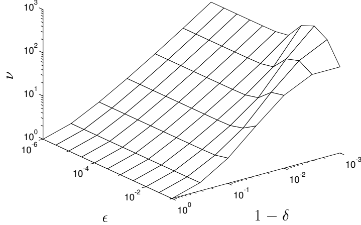
Figure 6: One way to measure non-normality. See text.
