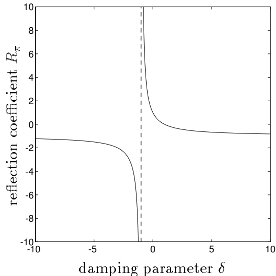
Figure 1: Dependence of the reflection coefficient on the damping parameter \delta .
