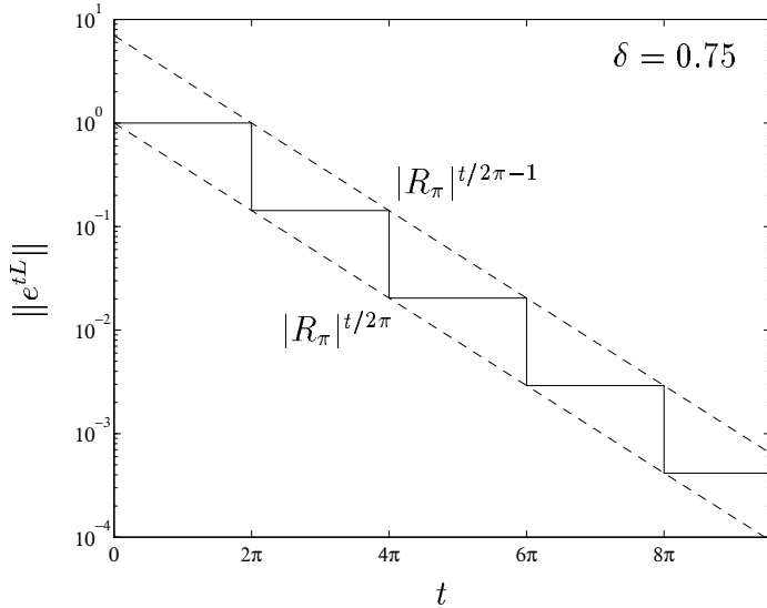
Figure 2: Exact solution operator norm (solid) and eigenvalue envelopes (dashed) for \delta = 0.75 . The lower envelope is given by (20) and the upper envelope is a constant multiple of the lower one, given by equation (26) in Section 4. Here the damping parameter is \delta = 0.75 ; with \delta = 1 , the norm drops to 0 at t = 2\pi .
