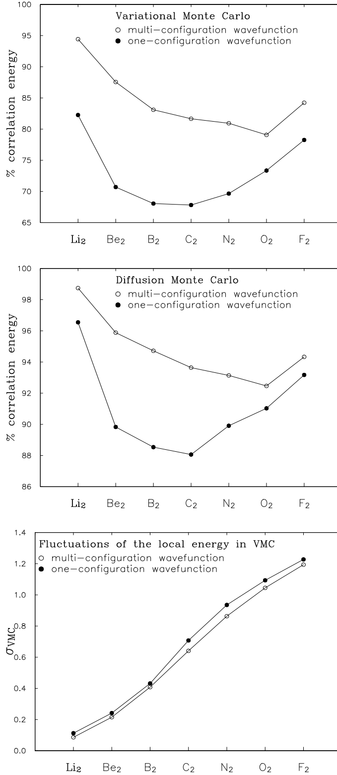
FIG. 1. Percentage of correlation energy in variational Monte Carlo (upper plot) and diffusion Monte Carlo (middle plot) and root-mean-square fluctuation \sigma_{\text{VMC}} (lower plot) with one-configuration (full circle) and multi-configuration (empty circle) wave functions. (Taken from Ref. 14.)
