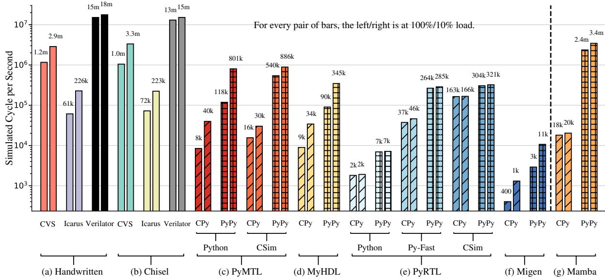
Figure 4.1: Simulation Performance Comparison of Different Hardware Development Workflows – Simulator performance for a 64-bit radix-4 iterative divider implemented at the register-transfer level. Results for identical random inputs for 1B cycles assuming the divider is active: (1) 100% of the time; and (2) only 10% of the time. Chisel = Chisel-generated Verilog; Handwritten = hand-written Verilog; CVS = commercial Verilog simulator; CSim = hybrid C/C++ compiled simulation; CPy = CPython. See Section 4.6 for details on the simulation platform.
