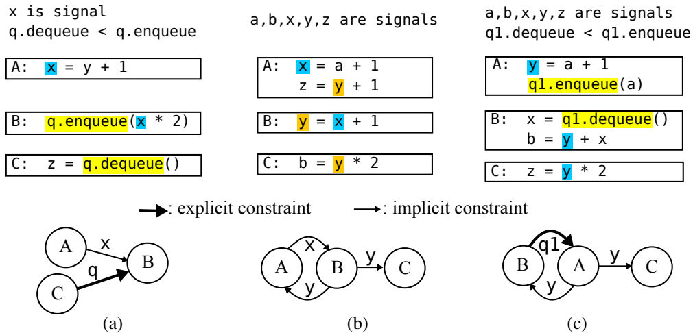
Figure 3.2: CL and RTL Process Examples using UMOc – Code of CL/RTL processes and corresponding unified directed graphs: (a) CL/RTL constraints can co-exist; (b) cycle of RTL processes; (c) cycle of CL processes.
