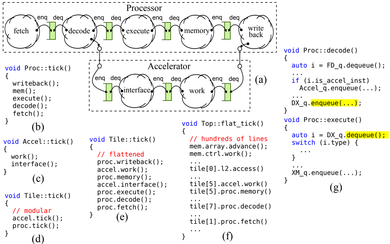
Figure 3.1: Modeling a Cycle-Level Processor/Accelerator Tile – An example abstracted from real-world simulator code: (a) the pipeline structure and composition of a five-stage processor and a two-stage tightly coupled accelerator where the accelerator request is sent out at decode and the response is accepted at writeback ; (b–c) the tick methods of Proc class and Accel class, both of which model pipeline behavior; (d) the modular tick method of Tile that calls the tick of Proc and Accel ; (e) the flat tick method that directly calls the hardware logic inside Proc and Accel for more accurate performance modeling; (f) the hypothetical flat tick function of a complex design that models the performance accurately; (g) Proc::decode and Proc::execute communicate through buffer DX_q .
