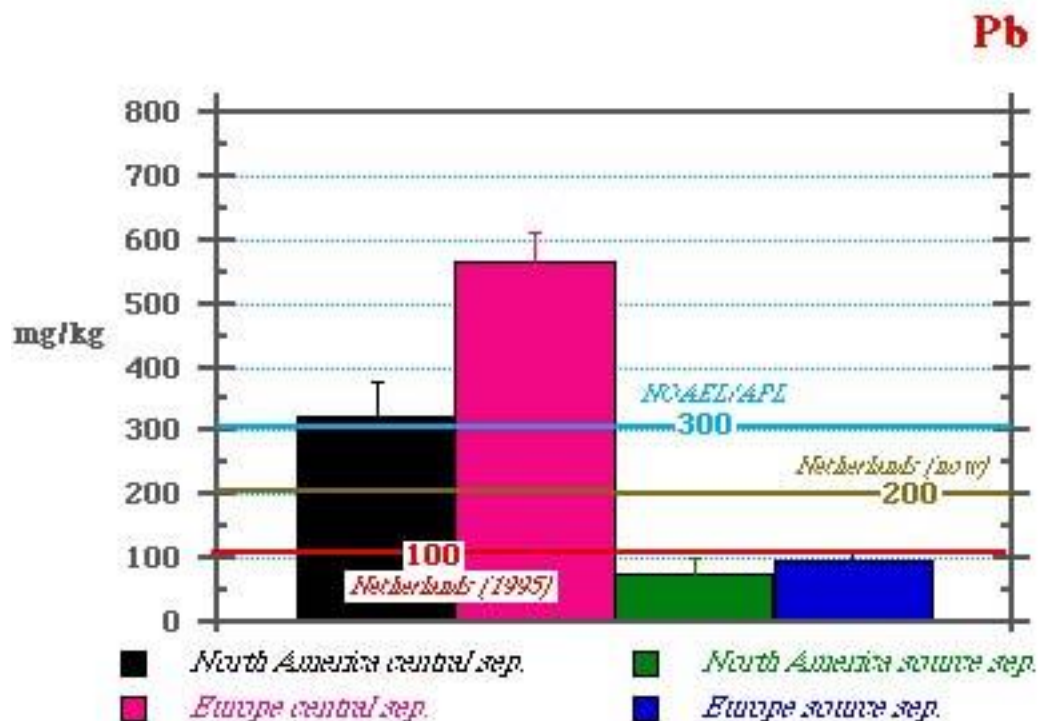
Figure 2. Average lead (Pb) levels in MSW composts from facilities using centralized separation to remove contaminants versus source separation of organic compostables in North America and Europe. Proposed USEPA (NOAEL/APL) standards as well as regulatory limits from the Netherlands are included for comparative purposes.
