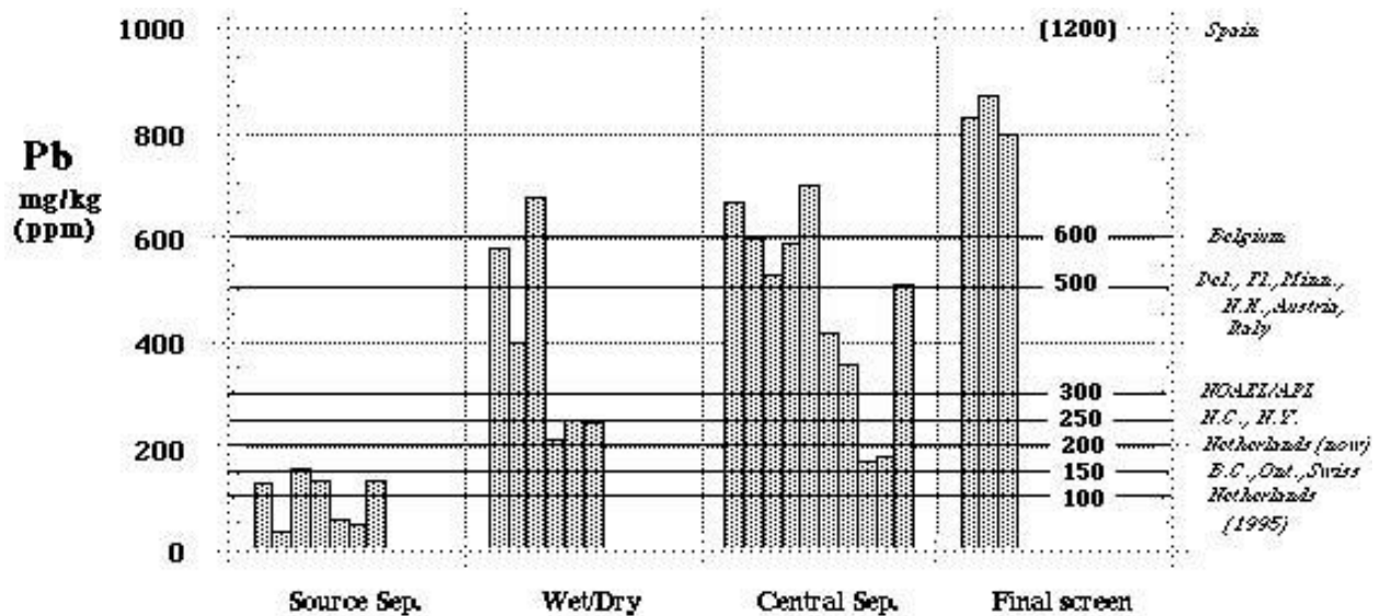
Figure 1. Lead (Pb) levels in MSW composts from experimental studies comparing several separation approaches. Regulatory standards from several U.S. states, Canadian provinces, and European countries are listed on the right axis.
