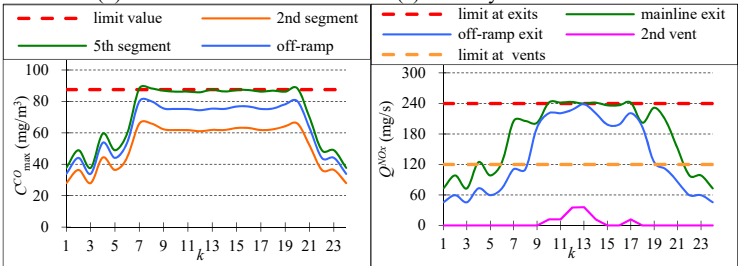
(d) C_{\max}^{CO} in tunnel segments (e) Q_{NO_x}^{NO_x} at discharge points Fig. 6. Tunnel ventilation control (with both C_{\lim}^{CO} and Q_{\lim}^{NO_x} targets)
