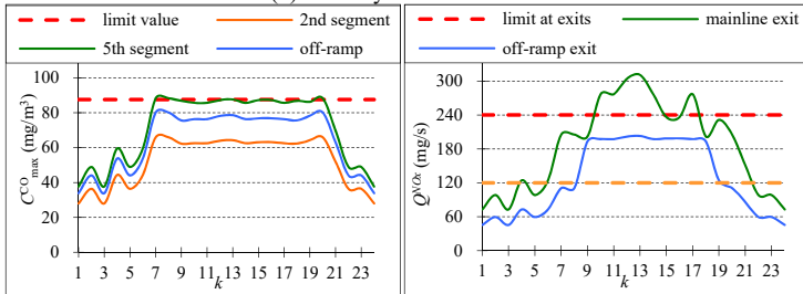
(c) C_{\max}^{CO} in tunnel segments (d) Q_{NO_x}^{NO_x} at discharge points Fig. 5. Tunnel ventilation control (with C_{\lim}^{CO} requirements)
