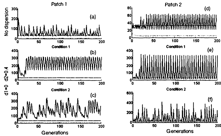
Figure 5: Behavior of patches 1 and 2 with different initial conditions.
