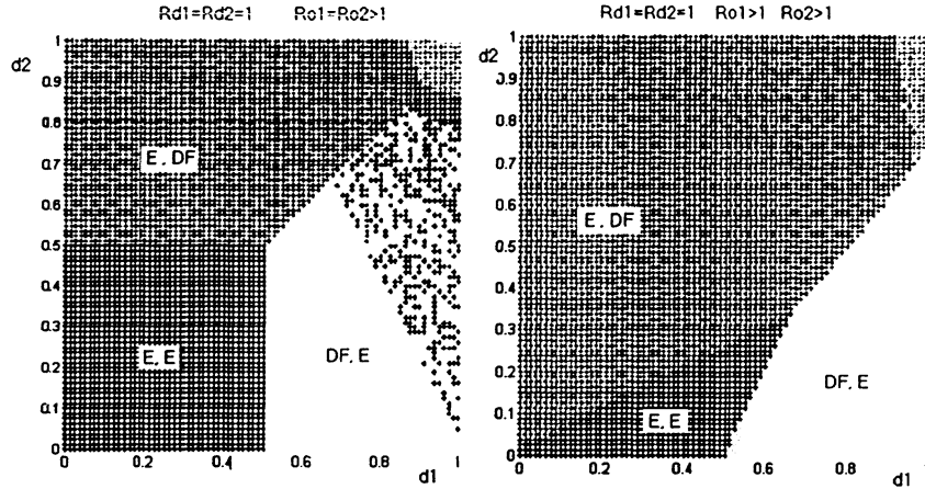
Figure 2: In this figure we observe symmetric behavior when disease and population dynamics are the same in both patches. The symmetry is broken when the R_{0_i} 's are different. The points in the upper right corner of both graphs are points that diverge or become negative; they are indicative of a Hopf Bifurcation.[4]
