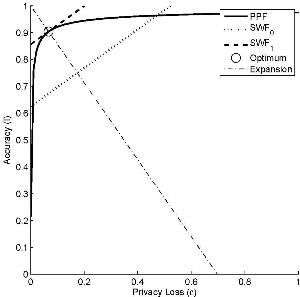
Figure 1 Publishing Income Data with Differential Privacy
