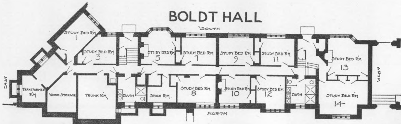
GROUND-FLOOR-PLAN
