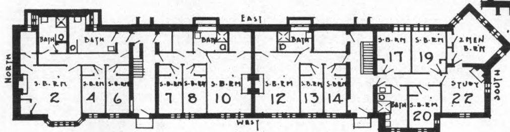
• GROUND-FLOOR-PLAN •
