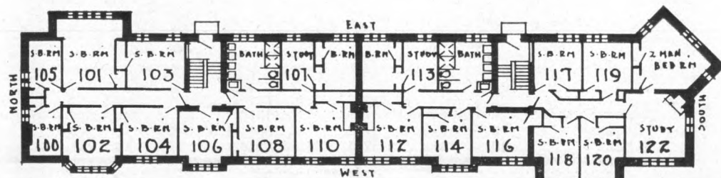
• FIRST-FLOOR-PLAN •
