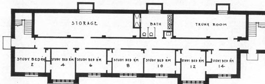
GROUND FLOOR PLAN MENNEN HALL
