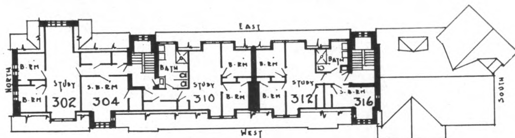
· THIRD-FLOOR PLAN ·
