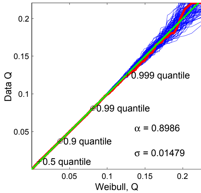
Figure 1: FIGURE 4B: Q-Q analysis (red curve). of the data from Figure 1 compared to a Weibull distribution (with parameters shown, estimated by quantile matching). Blue envelope shows this Weibull distribution gives an acceptable fit.
