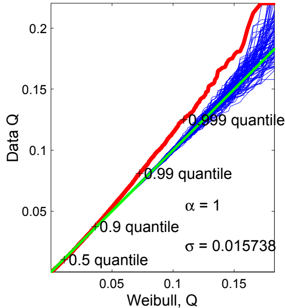
FIGURE 4A: Q-Q analysis (red curve). of the data from Figure 1 compared to an Exponential distribution (with parameters shown). Blue envelope shows sample variability, making it clear that the Exponential distribution is a poor fit.
