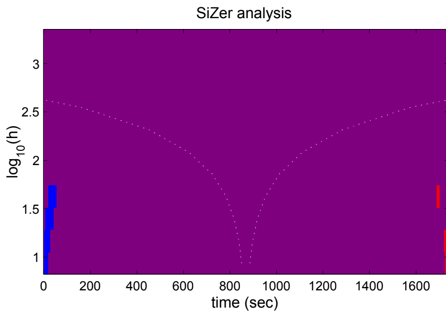
FIGURE 5: SiZer analysis.
