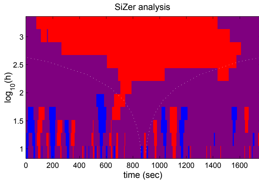
FIGURE 6: SiZer analysis.
