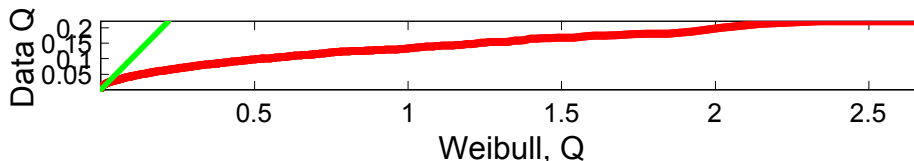
FIGURE 7: Q-Q analysis.
