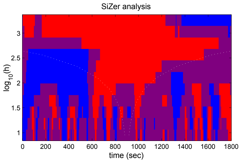
FIGURE 8: SiZer analysis.
