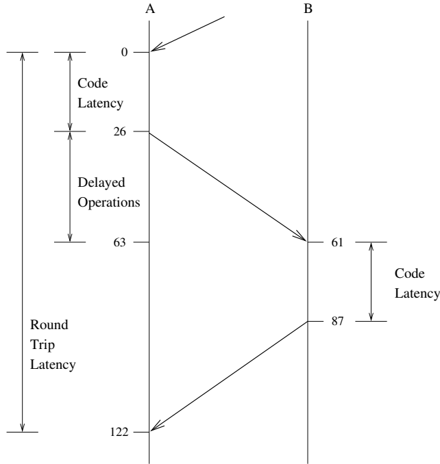
Figure 6: Round-trip latency time-line between two processes. Vertical scale is in \mu s .
