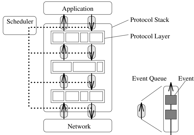
Figure 2: Elements of the layering model.
