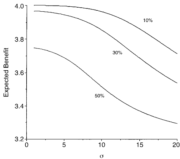
FIG. 2. Expected benefits accrued by an herbivore from feeding on a plant (see Fig. 1) as a function of the square root of the variance. Plants are heterogeneous and produce levels of toxins described by frequency distributions rather than single values. We assume that the level of toxin is normally distributed, with mean equal to 10%, 30%, or 50% of the fatal level and variance \sigma^2 . Under these conditions, benefits to herbivores decrease as the variance in toxin level increases.
