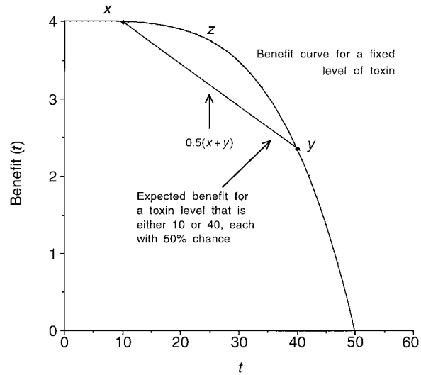
FIG. 1. We assume that the benefit B(t) an herbivore accrues from feeding on a plant is a decreasing function of the toxin t produced by the plant. (For the computation here, we used B(t) = \max(0, 4[1 - (t/50)^4]) so that t = 50 is a fatal level of toxin.) A plant that produces a variable level of toxin will lead to consistently lower levels of benefit than a plant that produces the mean level. For example, imagine a plant that produces 10 units of toxin with probability 0.5 and 40 units of toxin with probability 0.5. This corresponds to a variable plant (or plant tissue) that produces 10 units of toxin half the time and 40 units the other half. The corresponding benefits are x and y and the average benefit is 0.5(x + y) . The benefit z associated with the average level of toxin, 25 units, is larger than this average benefit (top arrow in Fig. 1). Thus, herbivores will have reduced success on plants that vary in their levels of defense compared to those with the same mean levels of toxin but less variability. If herbivore behavior reflects performance, an herbivore will prefer to feed on a plant that produces the constant level of toxin.
