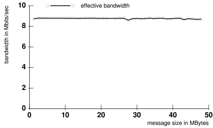
Figure 5: The effective bandwidth of URTP.
