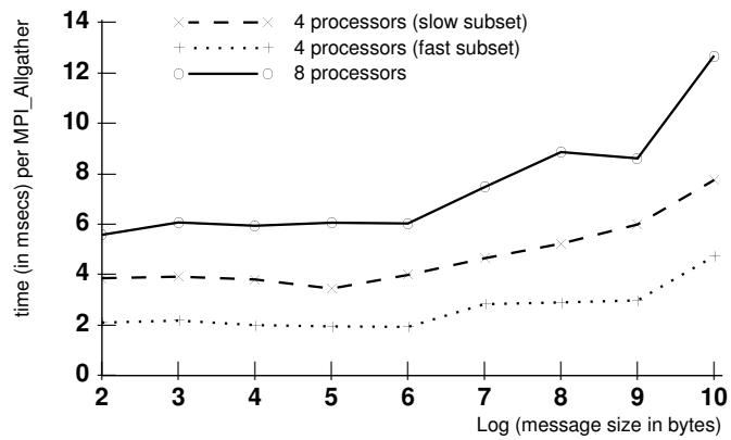
Figure 9: The time of MPI_Allgather (Algorithm 2, k = 1 ) as a function of the message size.
