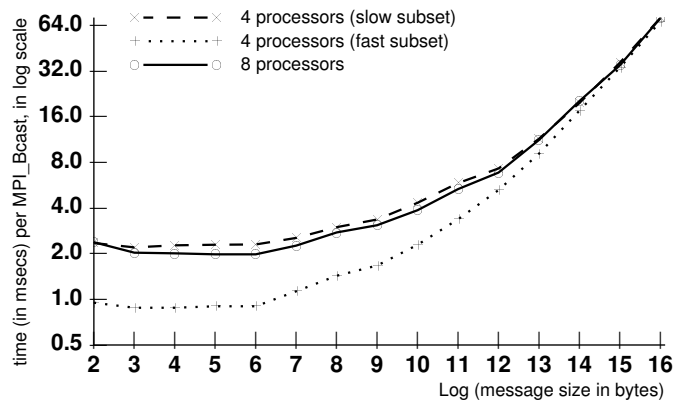
Figure 6: The time of MPI_Bcast as a function of the message size.
