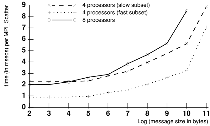
Figure 13: The time of MPI_Scatter as a function of the message size.
