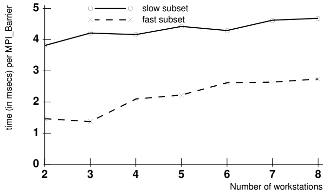
Figure 16: The time of MPI_Barrier as a function of the number of workstations.
