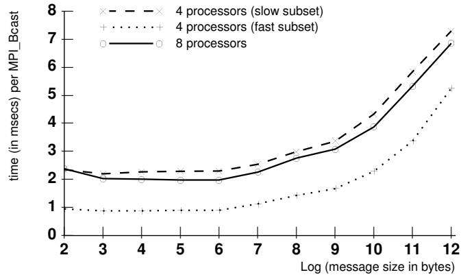
Figure 7: The time of MPI_Bcast as a function of the message size.
