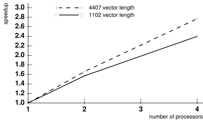
Figure 18: Speedup of sparse matrix-vector multiplication as a function of number of processors for two vector lengths using our MPI-CCL on URTP protocol.
