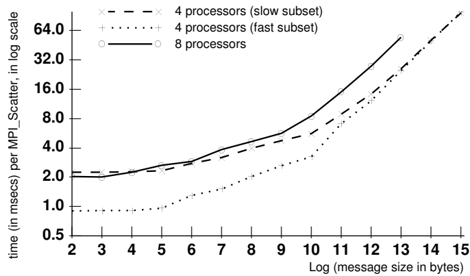
Figure 12: The time of MPI_Scatter as a function of the message size.
