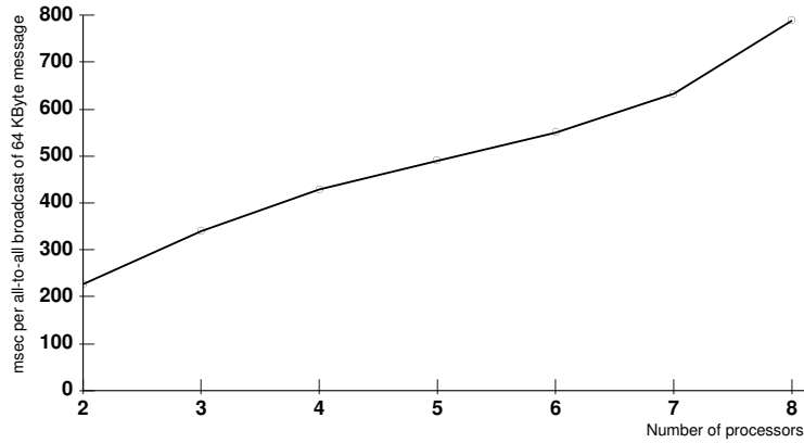
Figure 10: The time of MPI_Allgather (Algorithm 2, k = 1 ) as a function of the number of workstations using slow subset.
