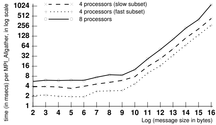
Figure 8: The time of MPI_Allgather (Algorithm 2, k = 1 ) as a function of the message size.
