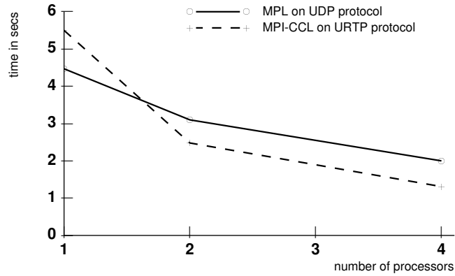
Figure 19: Performance of dense matrix-matrix multiplication using our MPI-CCL on URTP protocol versus that using IBM MPL product on LAN. The input matrices are 128 \times 128 .
