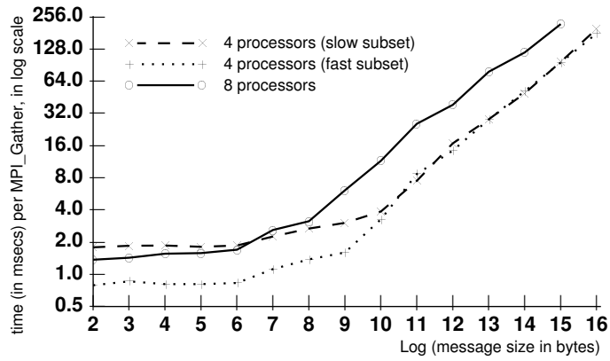
Figure 14: The time of MPI_Gather as a function of the message size.
