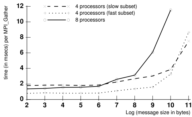
Figure 15: The time of MPI_Gather as a function of the message size.
