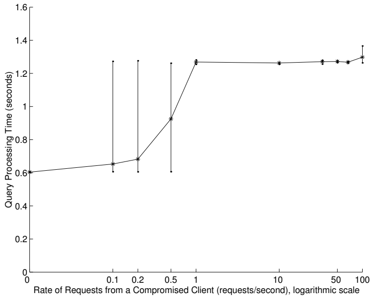
Figure 4: Performance of Query for a correct client when a compromised client makes requests at varying rates.
