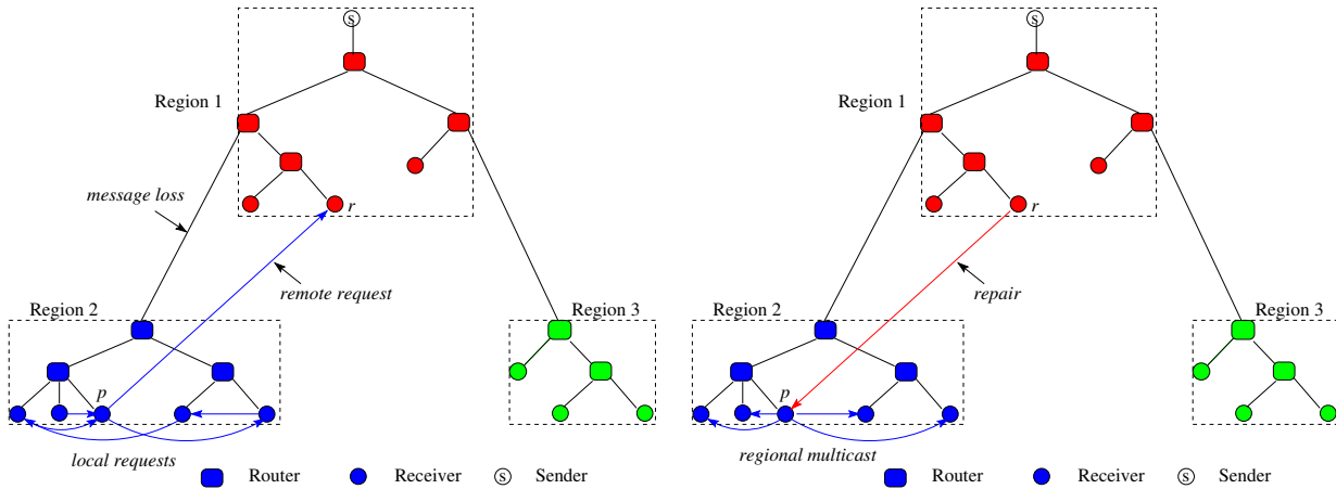
Fig. 3. Error recovery in RRMP
