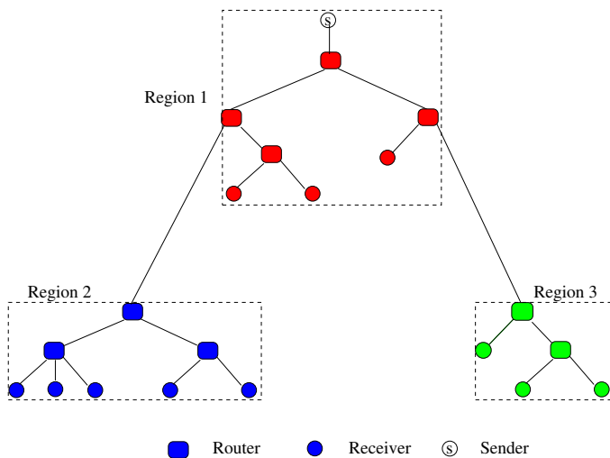
Fig. 2. Local regions in a hierarchical structure
