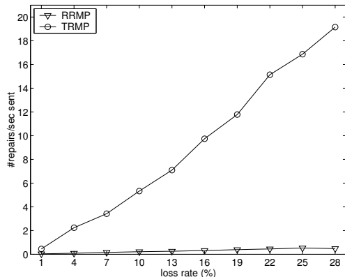
Fig. 8. Comparison of repair traffic for a lossy receiver
