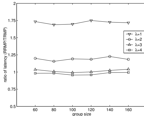
Fig. 9. Error recovery latency
