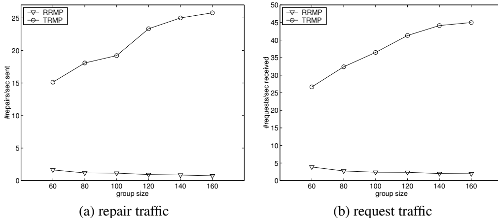
Fig. 7. Comparison of request and repair traffic when group size increases
