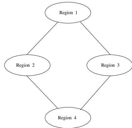
Fig. 6. Formation of error recovery hierarchy in RRMP. The parent region of a receiver in region 4 may contain a mixture of receivers from region 2 and receivers from region 3.
