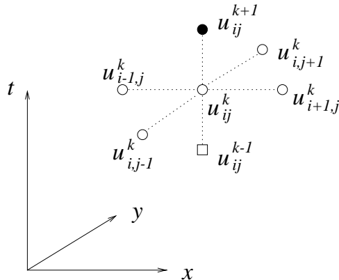
Figure 3: The stencil for the 2-D problem for an interior node. Boundary and corner nodes are slightly different and require separate treatment.
