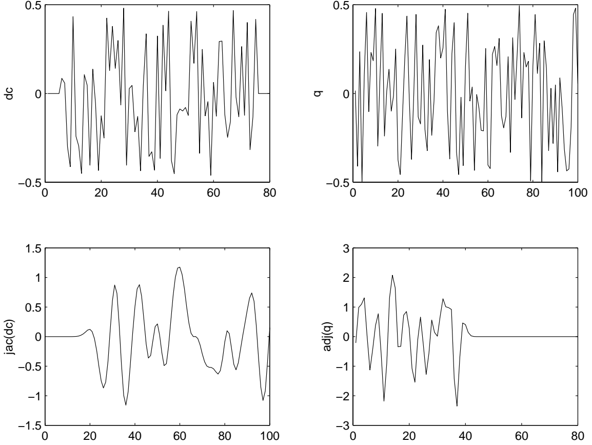
Figure 5: A test of the correctness of Jacobian and adjoint calculations. In this example, N = 80 and m = 100 . We choose at random 2 vectors d\mathbf{c} and \mathbf{q} displayed on the first row. On the second row, we show Jd\mathbf{c} and J^T\mathbf{q} . The inner products \mathbf{q}^T Jd\mathbf{c} and d\mathbf{c}^T J^T\mathbf{q} are evaluated. They agree to 14 digits.
