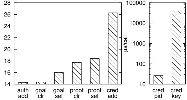
Figure 6: Authorization Control Overhead. Avoidance of cryptography reduces cost by 3 orders of magnitude.
