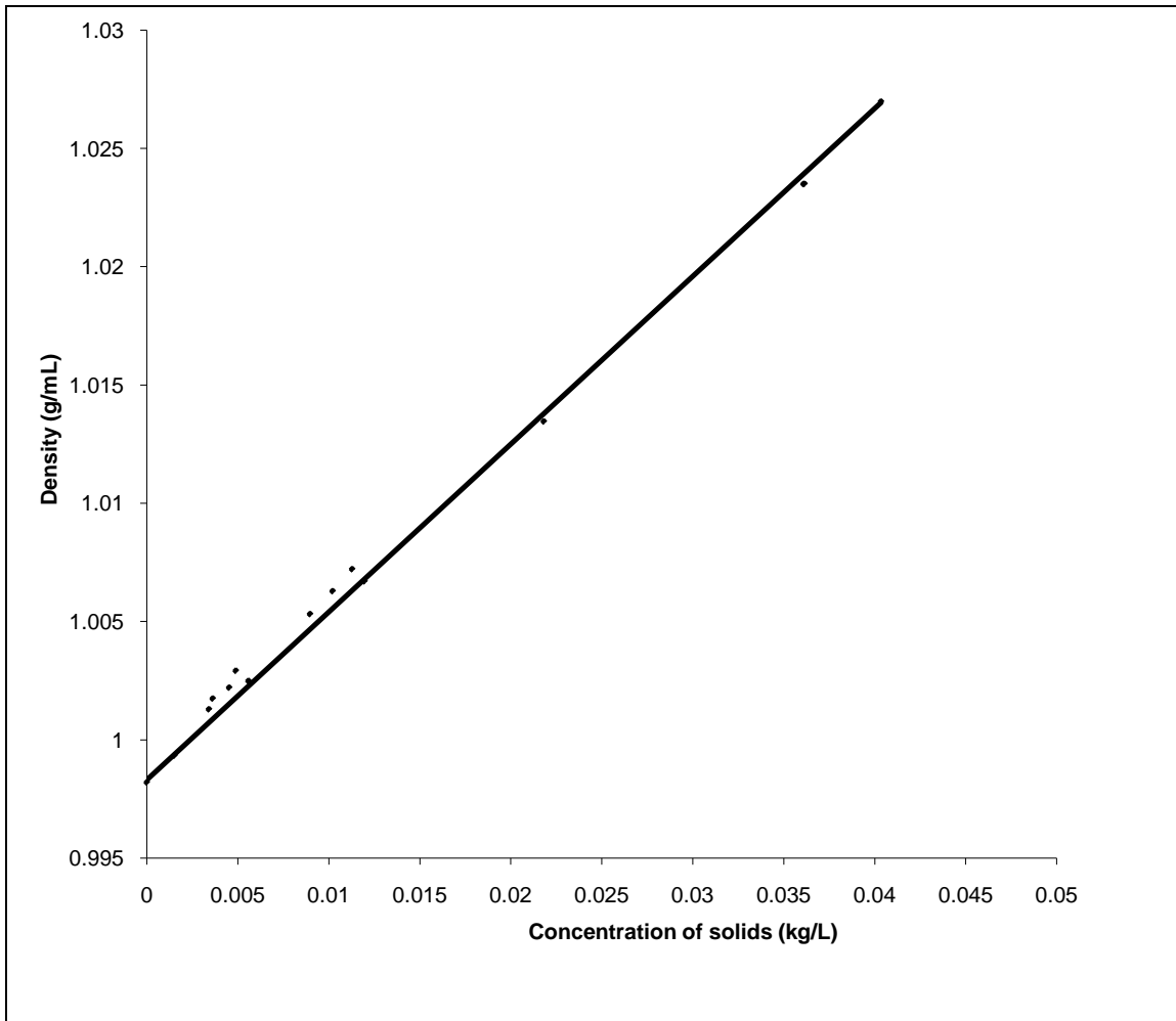
Figure 3-4. Relationship between floc blanket density and solids concentration ( r^2 = 0.98 ).
