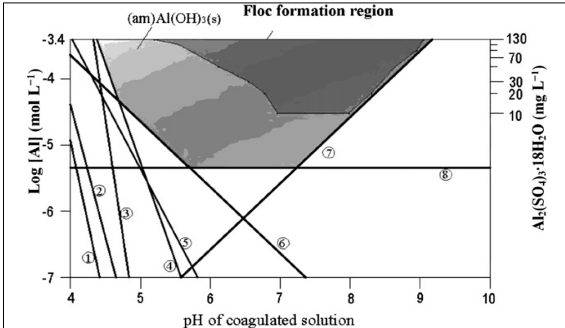
Figure 2-4. Aluminum solubility diagram in equilibrium with amorphous \text{Al}(\text{OH})_3(\text{s}) based on thermodynamic data, and floc formation region based on experimental observations. Lines 1, 2, 3, 4, 5, 6, 7, 8 represent the concentrations of [\text{Al}_3(\text{OH})_4]^{5+} , [\text{Al}_2(\text{OH})_2]^{4+} , [\text{Al}_{13}\text{O}_4(\text{OH})_{24}]^{7+} , \text{Al}^{3+} , \text{Al}(\text{OH})^{2+} , \text{Al}(\text{OH})_2^+ , \text{Al}(\text{OH})_4^- , \text{Al}(\text{OH})_3(\text{s}) , respectively (Xiao et al., 2008b).
