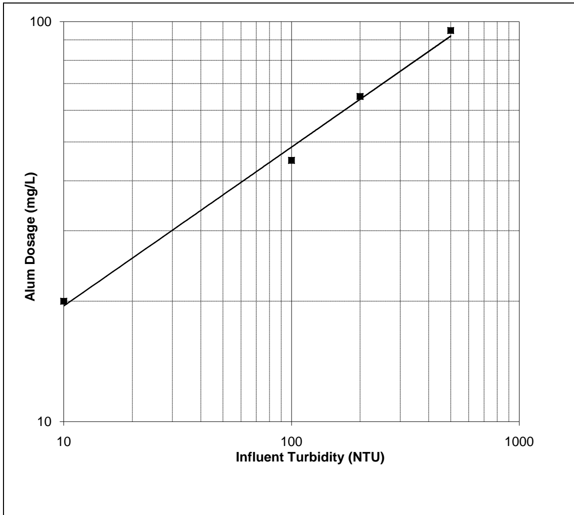
Figure 3-12. Empirical dosing model for the system studied.
