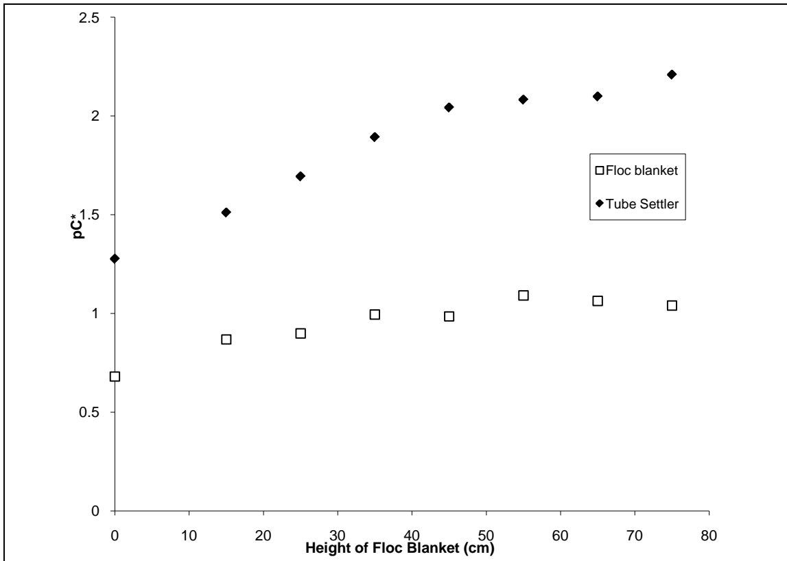
Figure 3-16. Effect of floc blanket height on removal efficiency from both tube settler and floc blanket effluents for flocculation conditions in the flocculator of G = 50 \text{ s}^{-1} and G\theta = 11500 .
