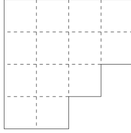
Figure 5.8: The shifted matroid determined by the facet \{3, 5, 7, 8\} .
