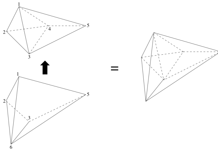
Figure 1.4: The second step in a convex-ear decomposition.
