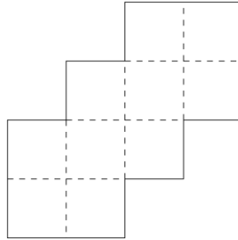
Figure 5.10: The lattice path matroid corresponding to [\{1, 2, 4, 6\}, \{3, 5, 7, 8\}] .
