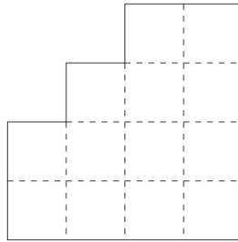
Figure 5.9: The reverse shifted matroid determined by the facet \{1, 2, 4, 6\} .
