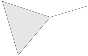
Figure 1.1: A simplicial complex with f-vector (1, 4, 4, 1) .
