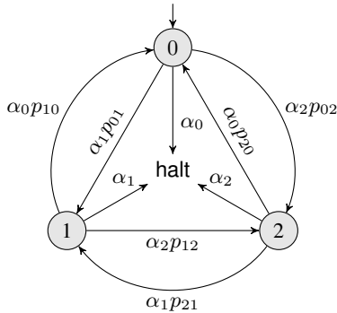
Fig. 4: A strictly deterministic automaton not equivalent to any while program
