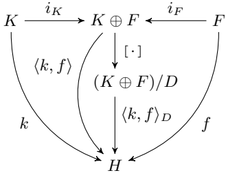
Fig. 1: Universality property of the commutative coproduct
