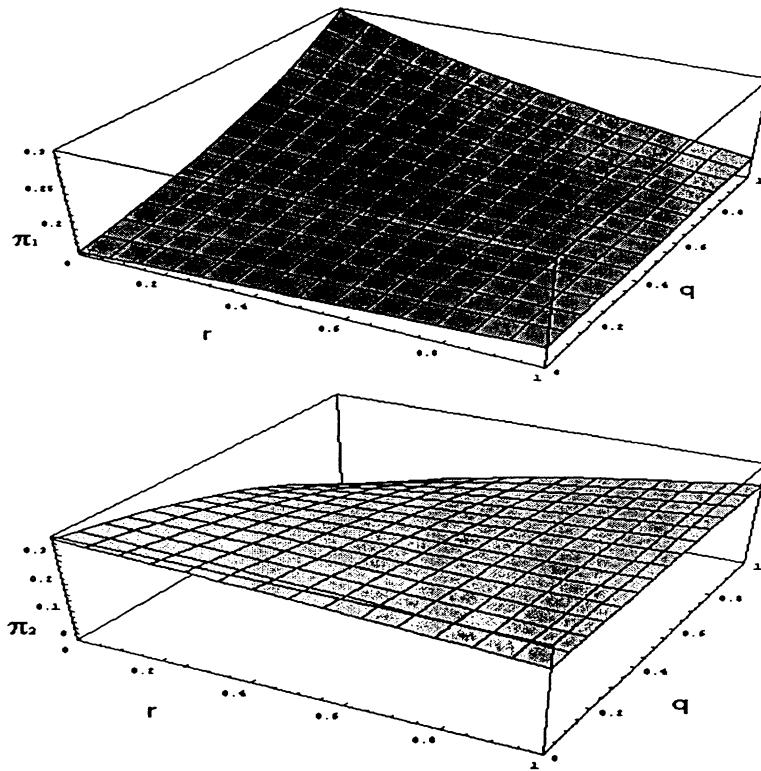
Figure 12: This is the probability plot of \pi_1 and \pi_2 when we vary r and q , and the child enters through X_0 .
