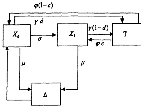
Figure 1: 4-State simulation, input into X_0
