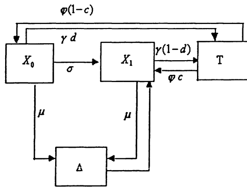
Figure 2: 4-State simulation, input into X_1
