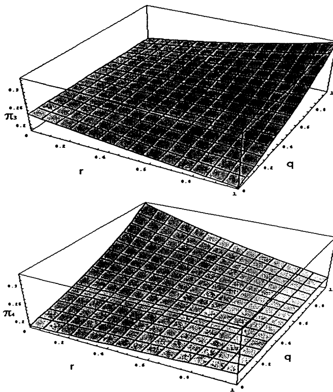
Figure 13: This is the probability plot of \pi_3 and \pi_4 when we vary r and q and the child enters through X_1 .
