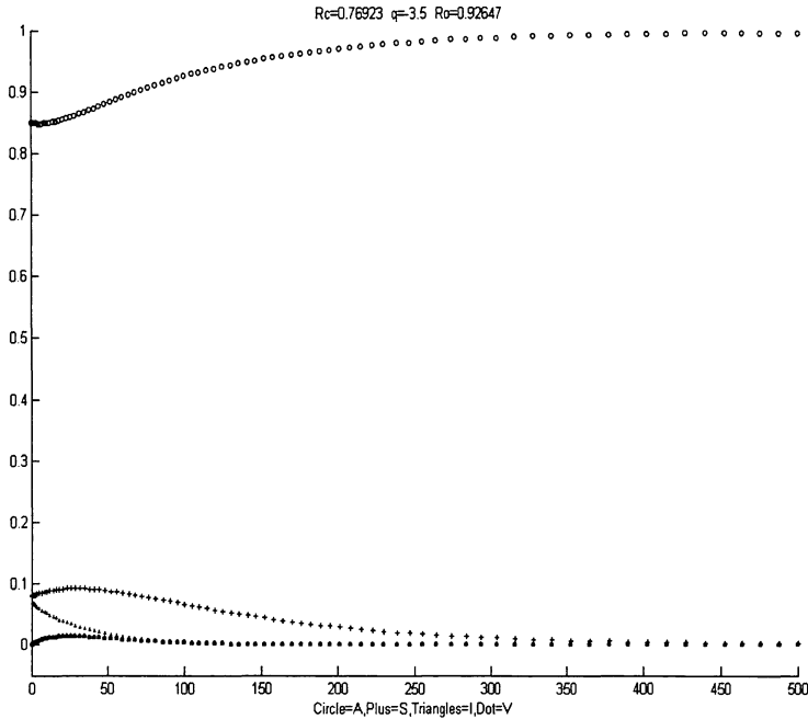
Figure 4: R_c < R_0 < 1
