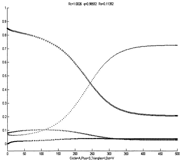
Figure 7: R_c > 1 and R_0 < 1
